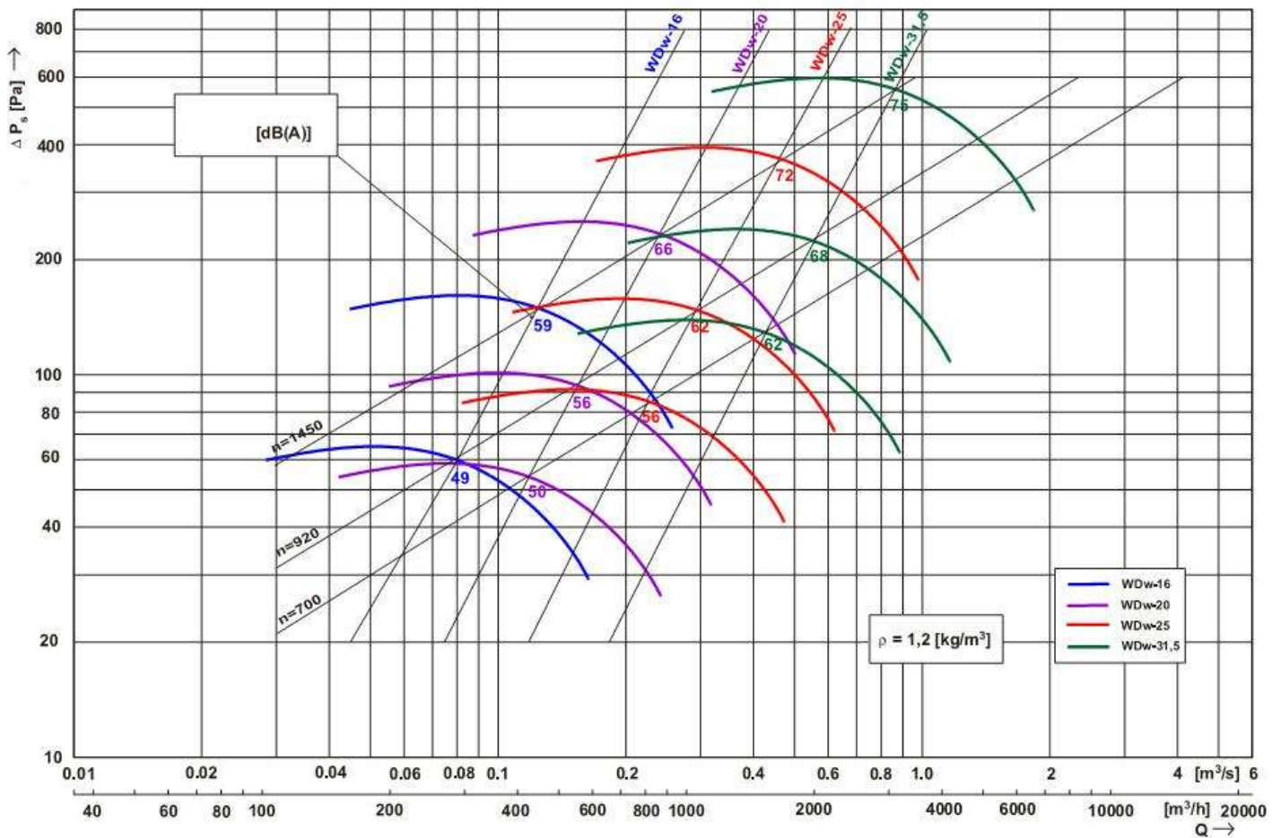
WDC W jelleggörbe
