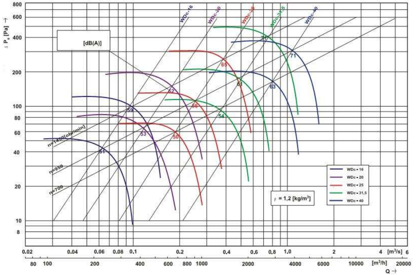
WDC W jelleggörbe
